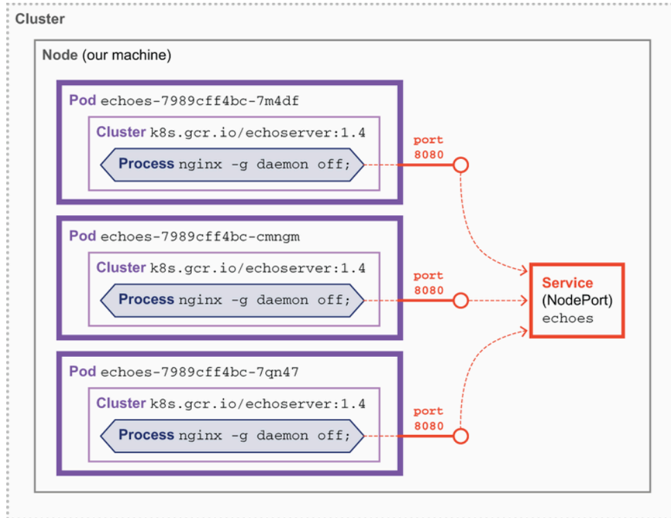
Figure 12.11 NodePort and services in the Kubernetes cluster
